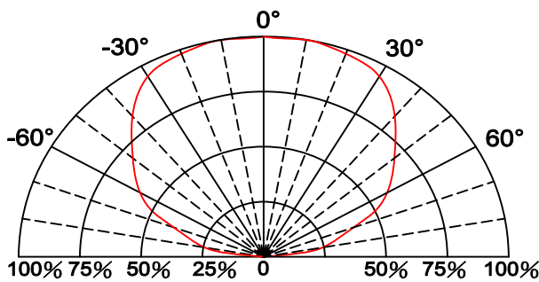
Fig.5 Directive Radiation
